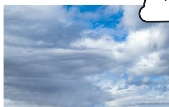
Stratocumulus
